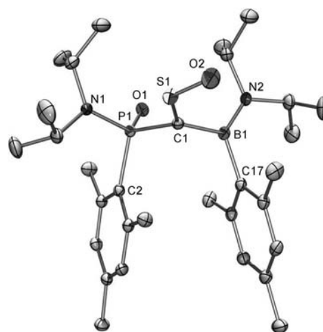
Figure 3. Molecular structure of 6 . Thermal ellipsoids set at 30% probability. H atoms are omitted for clarity.
